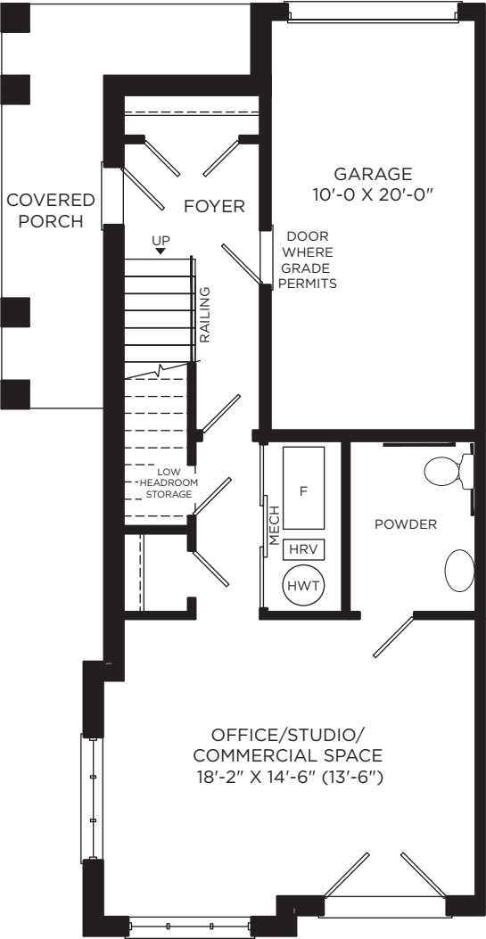
LOWER LEVEL
