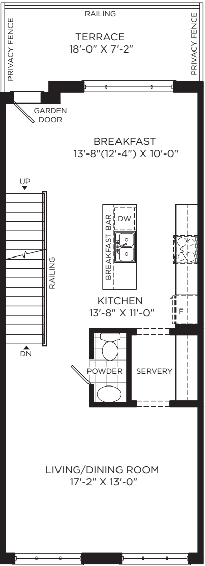
MAIN LEVEL
