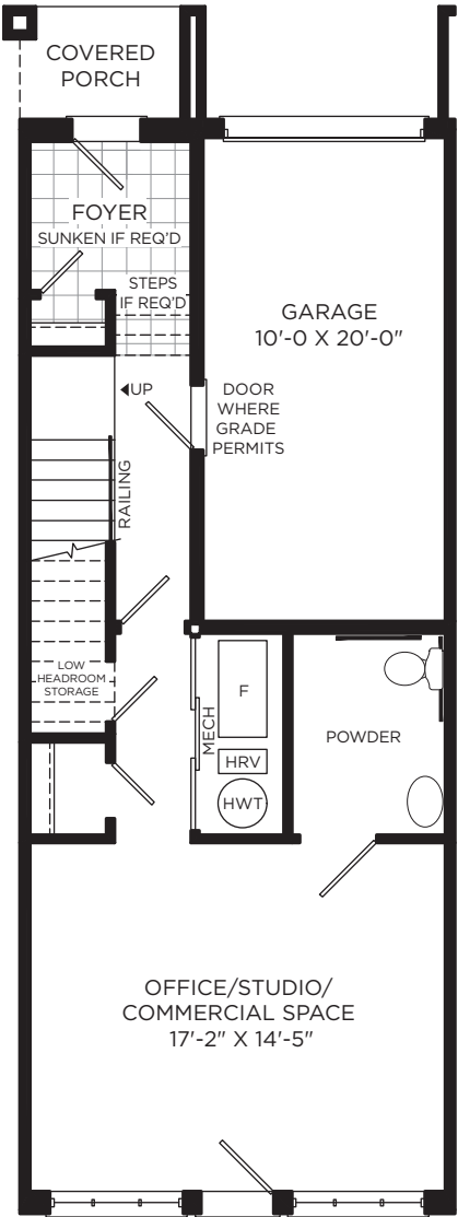
LOWER LEVEL
