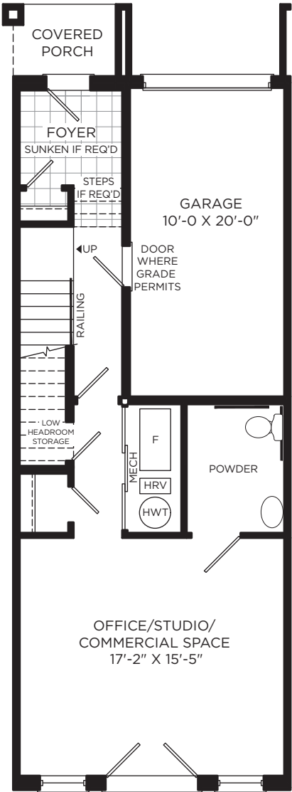
LOWER LEVEL
