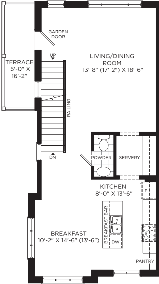
MAIN LEVEL
