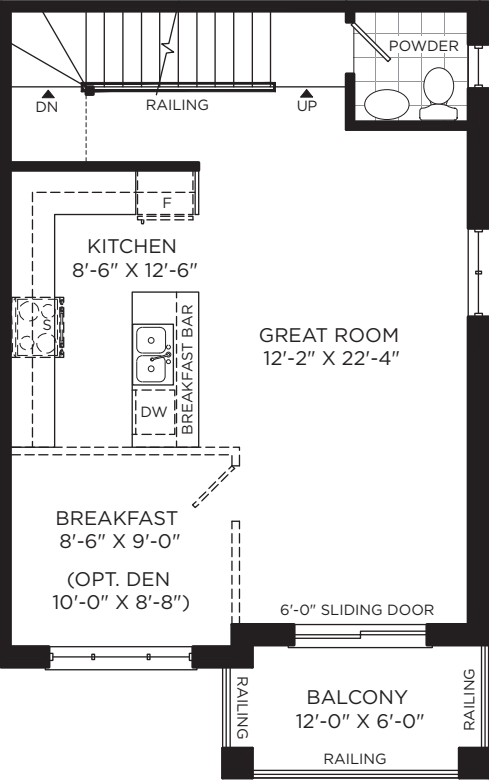
MAIN LEVEL
