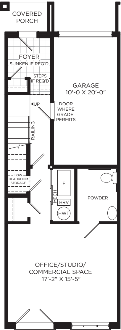
LOWER LEVEL
