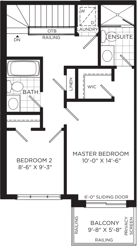
UPPER LEVEL
