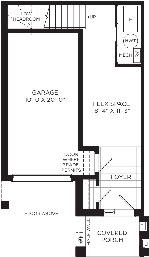
LOWER LEVEL
