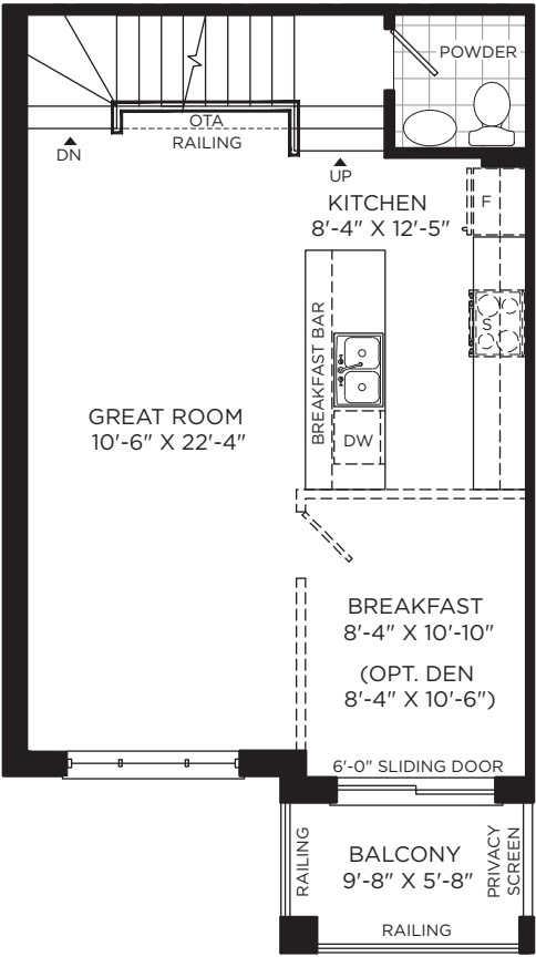
MAIN LEVEL
